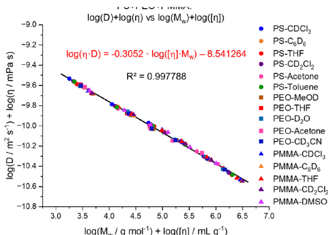
Figure 3. Dynamic viscosity corrected diffusion coefficients vs intrinsic viscosity corrected molar masses with Mark–Houwink parameters for PS, PEO, and PMMA in different solvents at T = 298.15 K.
