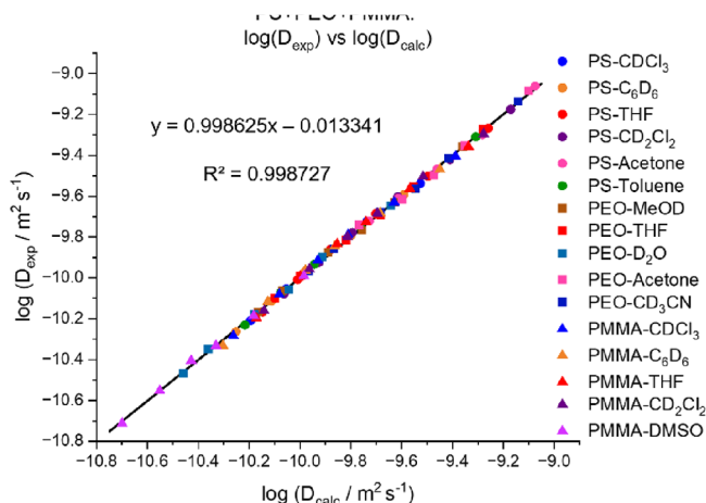
Figure 2. Experimental diffusion coefficients vs calculated diffusion coefficients via \log(D_{\text{exp}}) vs \log(D_{\text{calc}}) for PS, PEO, and PMMA in different solvents at T = 298.15 K.
