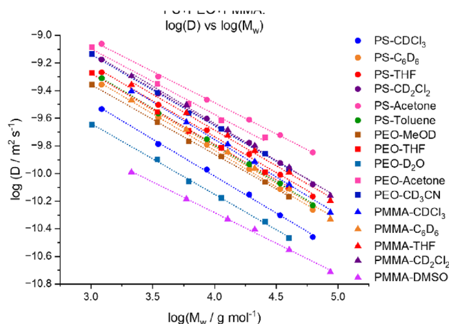
Figure 1. Diffusion coefficients vs molar masses for PS, PEO and PMMA in different solvents at T = 298.15 K.
